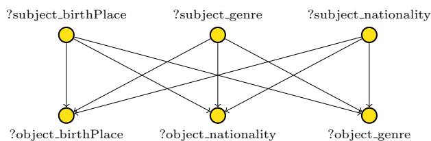
Fig. 7 The DBpedia query exhibiting treewidth equal to 3
