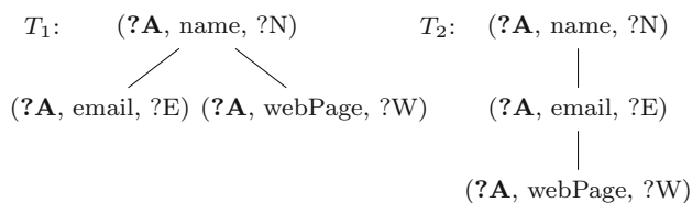
Fig. 4 Pattern trees that correspond to the queries in Example 2
