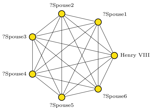
Fig. 9 The Henry VIII query, a 7-clique containing one constant and six variables. All edges between Henry VIII and the variables are labeled “dbpedia-owl:spouse,” and all edges between variables are labeled with the property path “dbpedia-owl:sameAs”
