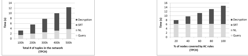
(a) Various total # of tuples; 100 nodes. (b) Various coverage of AC rules; 500 nodes, 500k tuples. Fig. 4. Query performance on uniform distributed data
