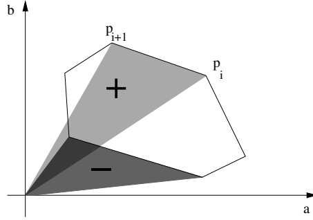
Fig. 2. Integration scheme over a polygonal domain.
