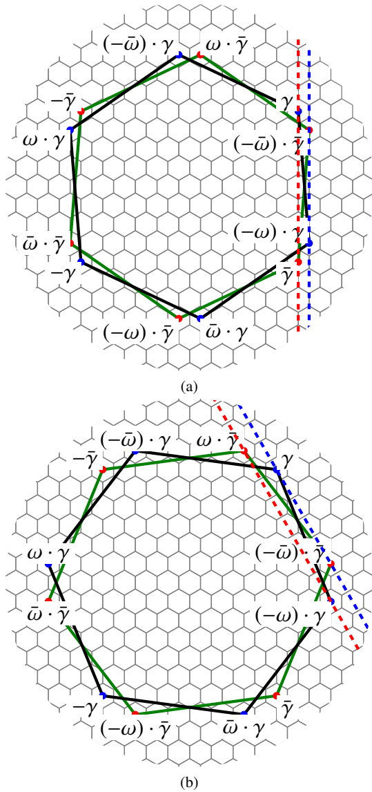
Fig. 9 Visualization of \mathcal{C}_{\gamma(2+\omega)}(0) and \mathcal{C}_{\bar{\gamma}(2+\omega)}(0) for the case: s > 0, t = s+1 (a) and s = 1, t > 1 (b). The two parallel lines discussed in the proof of Lemma 8 are illustrated by red and blue dashed lines
