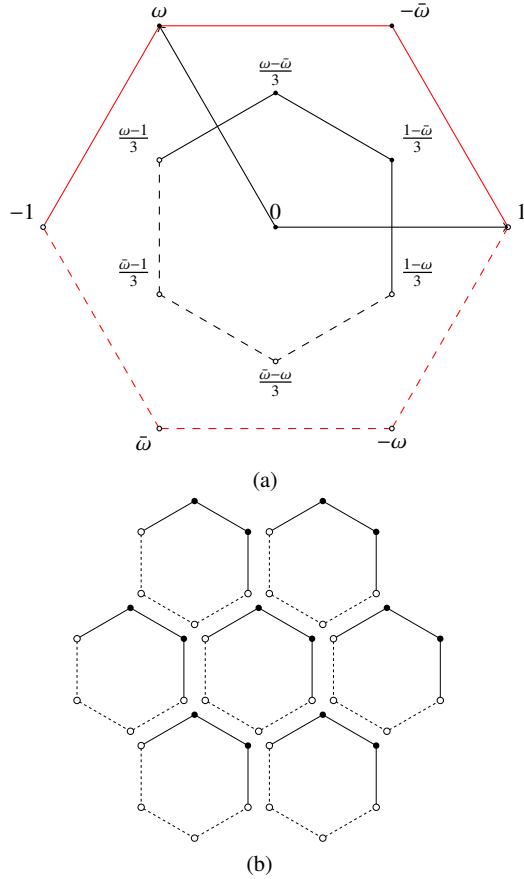
Fig. 4 In (a) visualization of hexagonal cells: \mathcal{C}_1(0) (in black) \mathcal{C}_{2+\omega}(0) (in red). Dashed lines and white circles—which represents points—are not included in hexagonal cells. (b) illustrates the adjacency of the sides and the vertices of hexagonal cells. The space between the hexagonal cells has been added for a visualization purpose.
