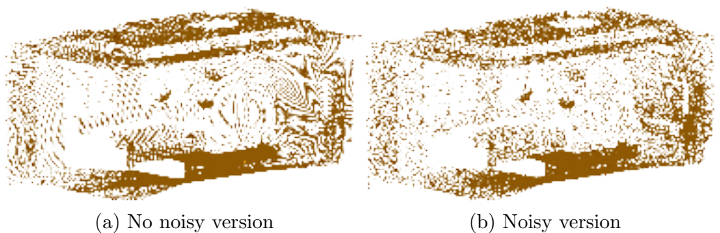
Figure 15: Point cloud obtained after a LiDAR scanner simulation in a CAD mesh model of an indoor scene called Living room 1.
