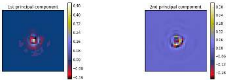
Figure 8: PCA-learned components.
