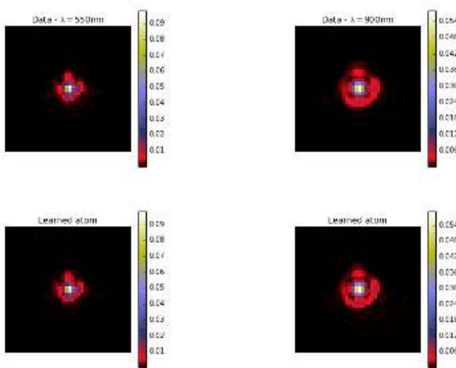
Figure 7: Extreme wavelength PSFs in the dataset and atoms making up the learned dictionary.
