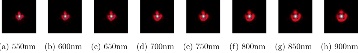
Figure 5: Simulated Euclid-like PSF variation at a fixed position in the field of view for varying incoming wavelengths.
