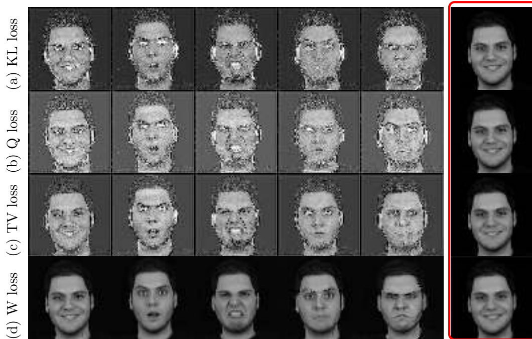
Figure 14. We compare the atoms (columns 1 to 5) obtained using different loss functions, ordered by the fidelity of the reconstructions to the input measures (using the mean PSNR), from best to worst: the KL divergence (a) \overline{PSNR} = 32.03 , the quadratic loss (b) \overline{PSNR} = 31.93 , the total variation loss (c) \overline{PSNR} = 31.41 , and the Wasserstein loss (d) \overline{PSNR} = 30.33 . In the last column, we show the reconstruction of the same input image for each loss. We notice that from (a) to (d), the atoms' visual appearance seems to increase even though the reconstruction quality decreases.
