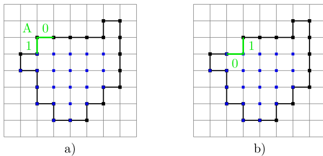
Fig. 8. (a) A is a point in the \mathcal{WN} -path, where its neighboring points back and forth in Bd_{\mathcal{WN}}(C) form the sub-word 10. (b) Removing the point A corresponds to switching the sub-word 10 into 01, i.e. applying the switch operator at the position of the point A.
