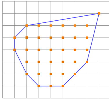
Fig. 3. An example of a digital set C that is digitally convex but not 4-connected. The orange points represent the elements x \in C while the blue line represents Conv(C) .
