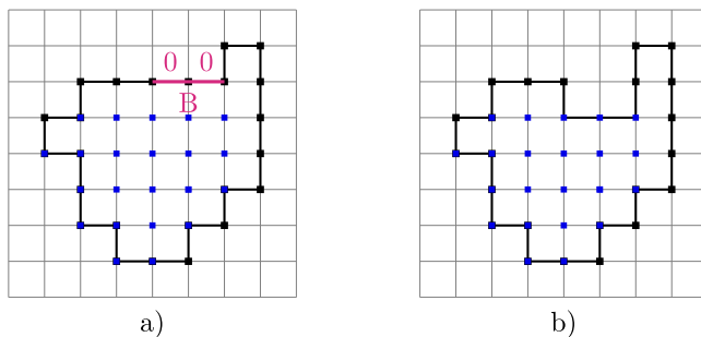
Fig. 9. (a) B is a point in the \mathcal{WN} -path, where its neighboring points back and forth in Bd_{\mathcal{WN}}(C) form the sub-word 00. (b) The digital convexity is lost when removing the point B.
