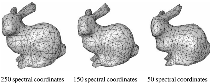
Figure 5. Spectral reconstruction of Bunny model (502 vertices) with different number of spectral coordinates.
