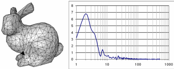
Figure 4. Bunny model and its spectral decomposition ( S_i for i=1 to i=502 ).
