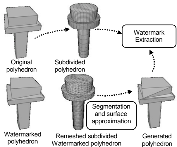
Figure 9. Mark extraction process for a subdivided polyhedron attacked by re-meshing
