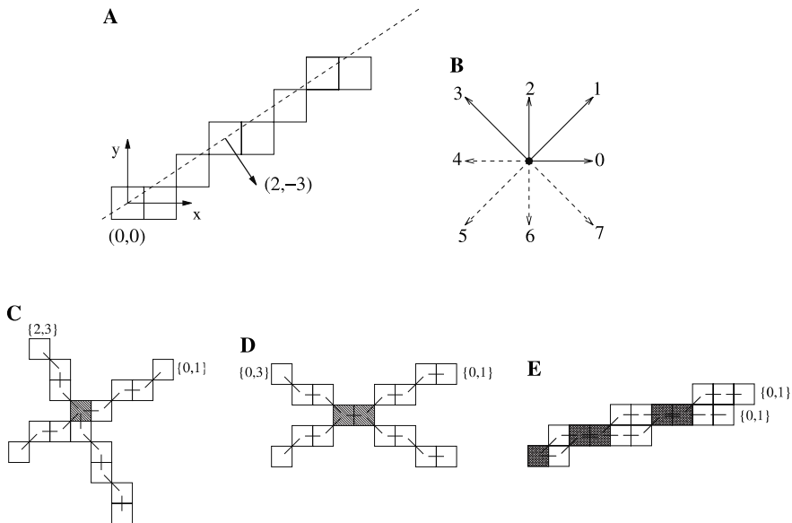
Fig. 1. (A) The digital naive line of parameters (a, b, \mu) = (2, -3, 0) ; (B) Chain codes; (C) two naive lines with no common direction; (D) two naive lines with one common direction; (E) two naive lines in the same octant; and (C–E) the Chain codes of those digital lines are also depicted.
