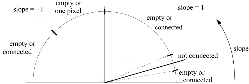
Fig. 2. Summary scheme: connectivity of the intersection of the bold line and lines with different slopes.
