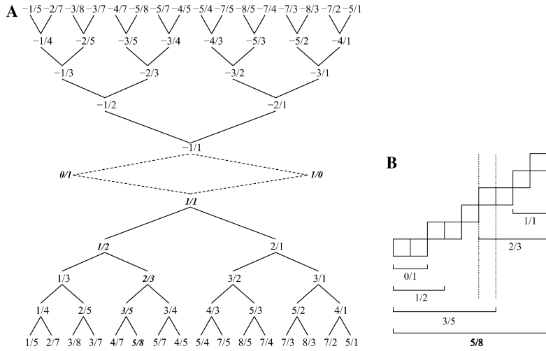
Fig. 6. (A) Stern-Brocot tree: positive and negative irreducible rational fractions. (B) Decomposition of one period of the digital line of slope \frac{5}{8} : for each fraction of the path in the Stern-Brocot tree, the corresponding set of pixels (one period) appearing in the period of the \frac{5}{8} slope digital line.
