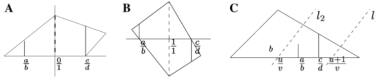
Fig. 5. Illustration of the three cases of Theorem 5.
