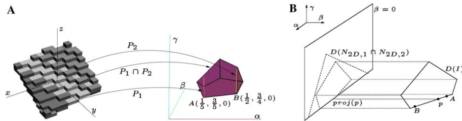
Fig. 8. (A) Preimage of the intersection of the digital naive planes P_1(1, 3, 5, 0) and P_2(2, 3, 4, 0) ; (B) illustration of the proof of Theorem 12.
