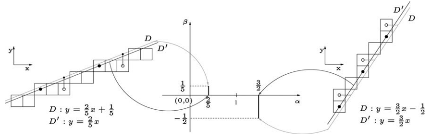
Fig. 4. On the left (resp. right), a digital straight line L_1 (resp. L_2 ) with parameters (2, -5, 0) (resp. (-3, 2, 0) ) and the Euclidean lines defining the set of lines whose OBQ digitization is L_1 (resp. L_2 ). In the middle, the preimages of L_1 and L_2 are vertical segments whose extremities are related to the lines D and D' on the left and on the right.
