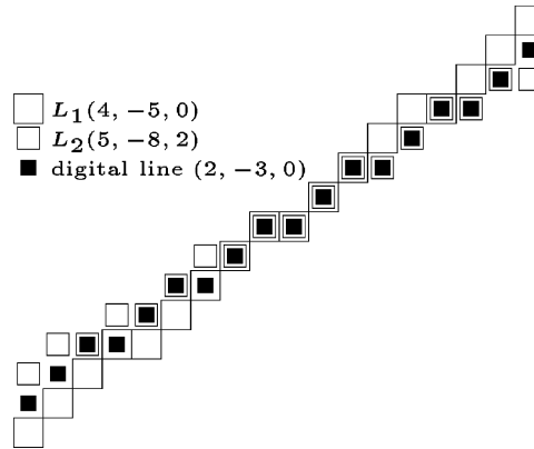
Fig. 3. Two digital lines L_1 and L_2 , and the digital line which parameters are the minimal parameters of L_1 \cap L_2 .
