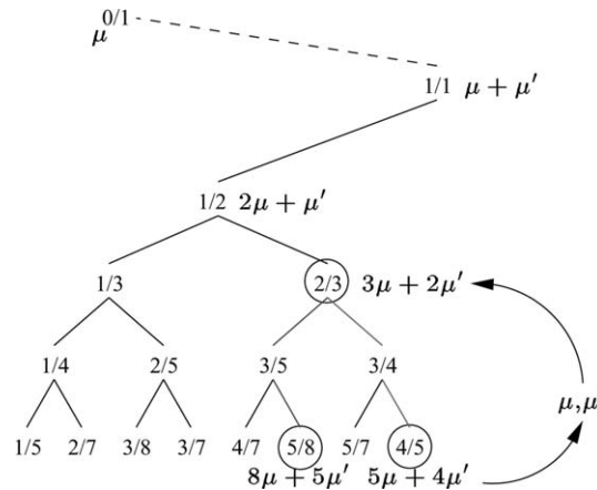
Fig. 7. Remainder calculation for the digital lines (4, -5, \mu_1) et (5, -8, \mu_2) : the two values \mu and \mu' are solutions of the system 8\mu + 5\mu' = \mu_1 , 5\mu + 4\mu' = \mu_2 , and then injected in the equation 3\mu + 2\mu' in order to get the remainder of the intersection.
