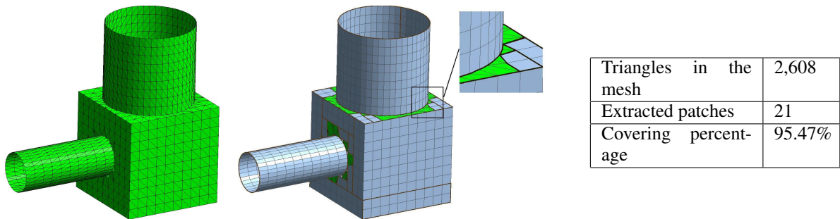
Figure 15: Original mesh and result for: CubeCylinders .
