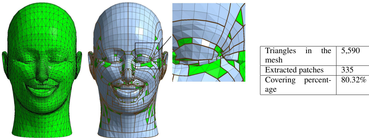
Figure 12: Original mesh and result for: Face .
