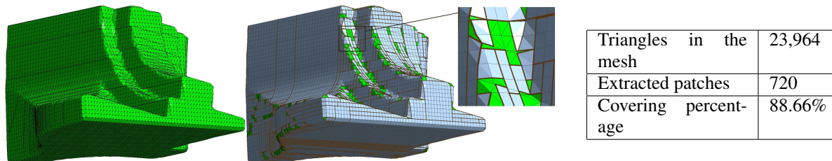
Figure 13: Original mesh and result for: Fandisk .
