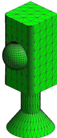
Figure 7: MeshObject3 : 1,712 triangles
