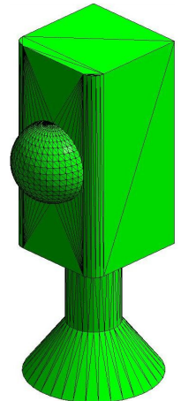
Figure 9: MeshObjectSparse : 1,034 triangles
