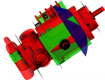
Figure 22: Extracted primitives
