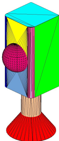
Figure 15: MeshTestSparse segmented
