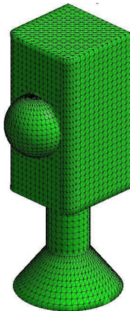
Figure 6: MeshObject2 : 6,434 triangles
