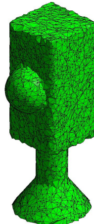
Figure 8: MeshObjectIrreg : 9,938 triangles
