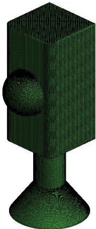
Figure 5: MeshObject1 : 55,318 triangles
