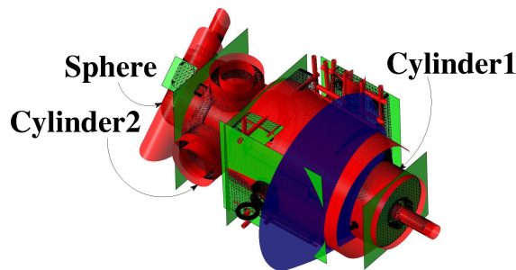
Figure 23: Extracted primitives
