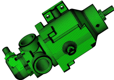
Figure 21: PumpMesh : 158,746 triangles
