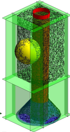
Figure 13: Primitives from MeshObjectIrreg
