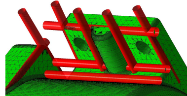
Figure 24: Zoom on some extracted cylindrical blends
