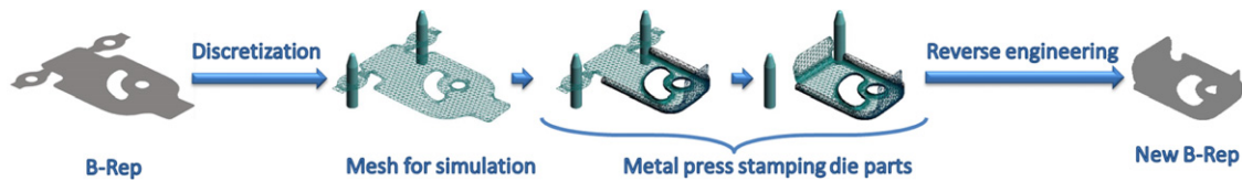
Fig. 1. The B-Rep model has to be discretized into a 3D CAD mesh in order to be processed by a metal press stamping die parts simulation, and no longer correspond with the final mesh.
