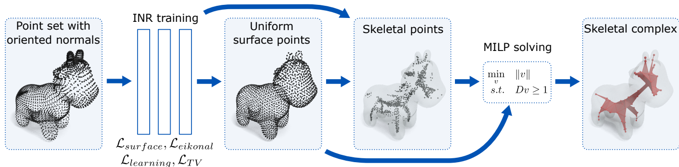
Fig. 2: Overview of our method. An implicit neural representation is trained on the input point set, uniform surface points and skeletal points are extracted, and the skeleton mesh is recovered using a cover-set formulation solved as a Mixed-Integer Linear Program (MILP).
