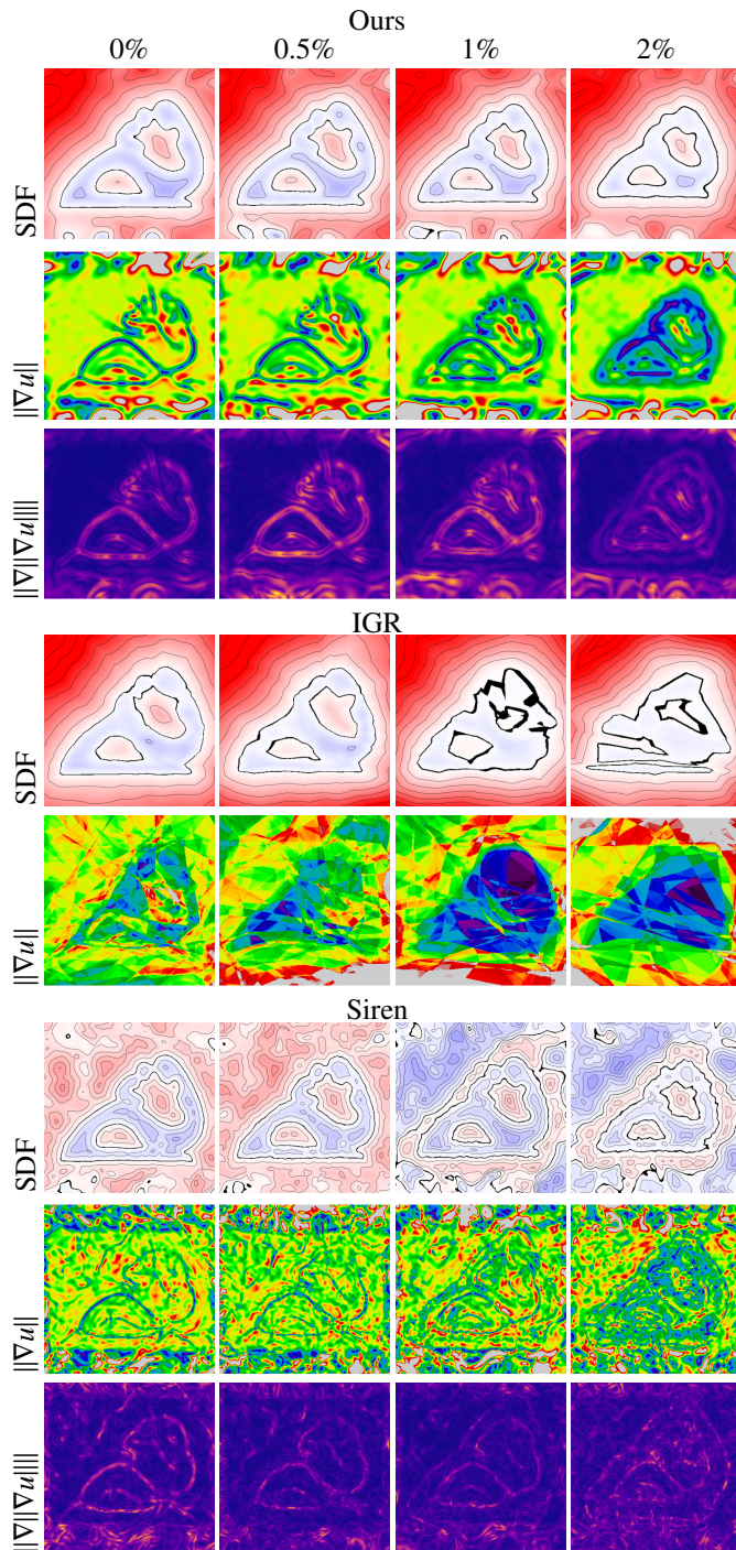
Fig. 13: Slices of the SDF and the gradient's norm of the fertility shape with increasing levels of noise for different INR (variances set to 0, 0.5, 1, and 2% of the shape diagonal). Since IGR's second order derivatives are 0, we do not show \|\nabla\|\nabla u\|\| for this method.
