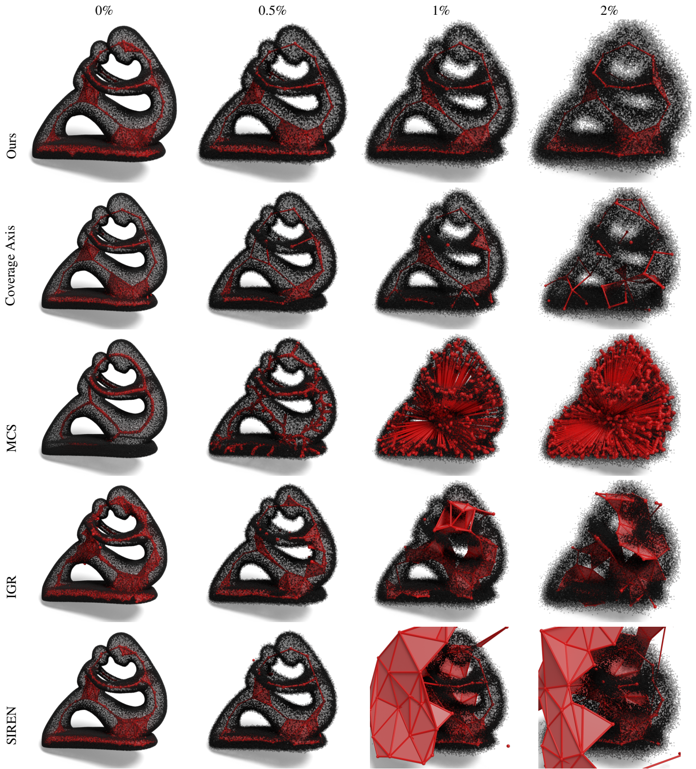
Fig. 12: Skeleton of the fertility shape with increasing levels of noise (variances set to 0, 0.5, 1, and 2% of the shape diagonal)
