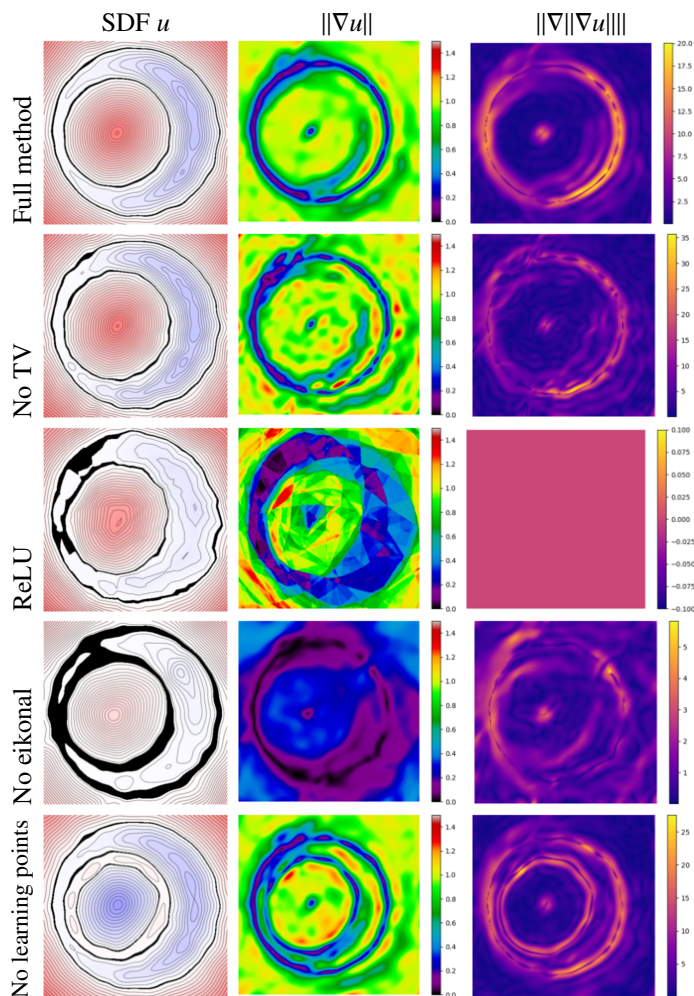
Fig. 10: Slices of u , \|\nabla u\| and \|\nabla\|\nabla u\|\| obtained by removing different parts of the loss.
