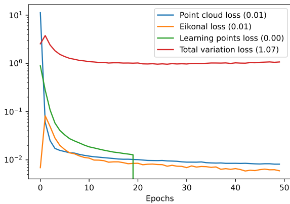
Fig. 11: Evolution of the different terms of the loss. After 20 epochs, we remove the learning points loss (Equation 5) to allow for more flexibility since in case of noise or missing data, the learning points might be inaccurate.
