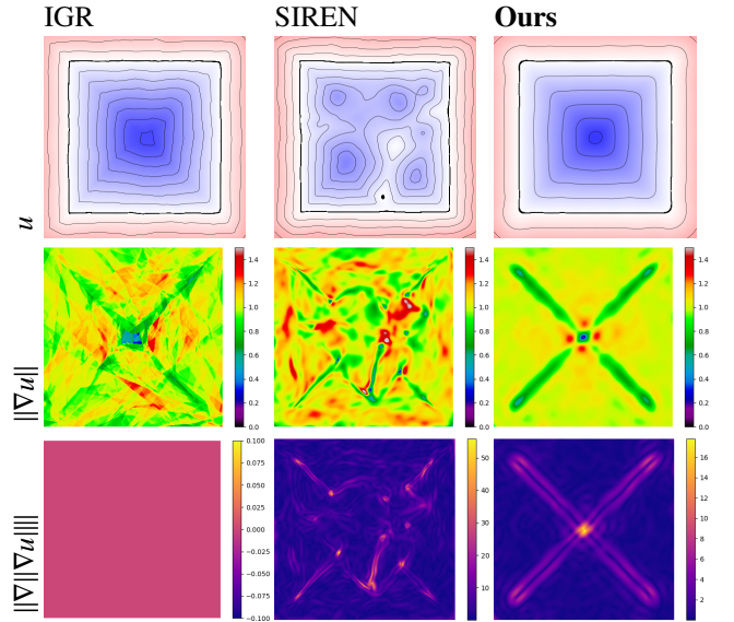
Fig. 3: Slices of the SDF, gradient’s norm and norm of the gradient’s norm, using IGR, SIREN and our TV-regularized method on a cube. IGR using ReLU activation function, the second order derivative is 0 almost everywhere.
