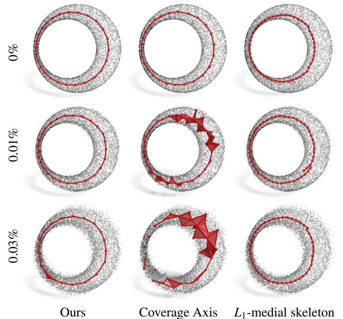
Fig. 8: Comparison with Coverage Axis and L_1 -medial skeleton on a torus with different levels of noise (no noise, 0.01% and 0.03% of the shape's diagonal).
