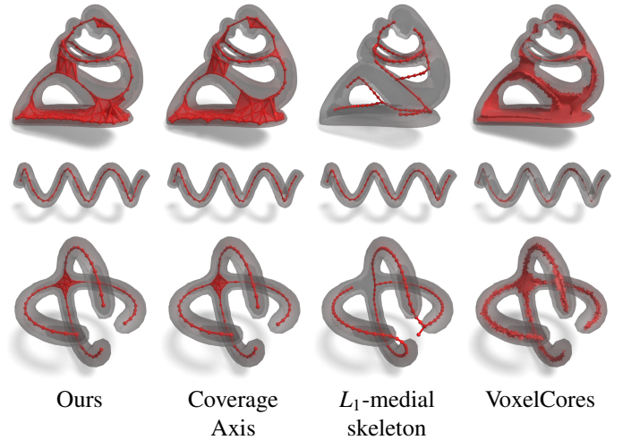
Fig. 4: Comparison with Coverage Axis, L_1 -medial skeleton and VoxelCores on standard shapes.
