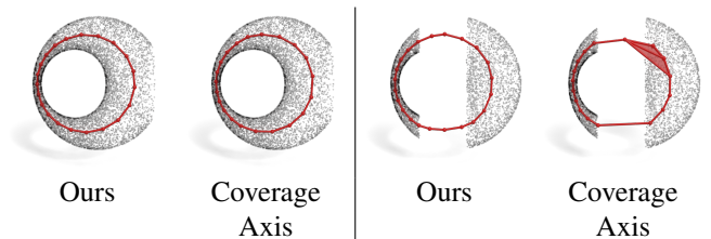
Fig. 9: Comparison with Coverage Axis on point clouds with missing data.
