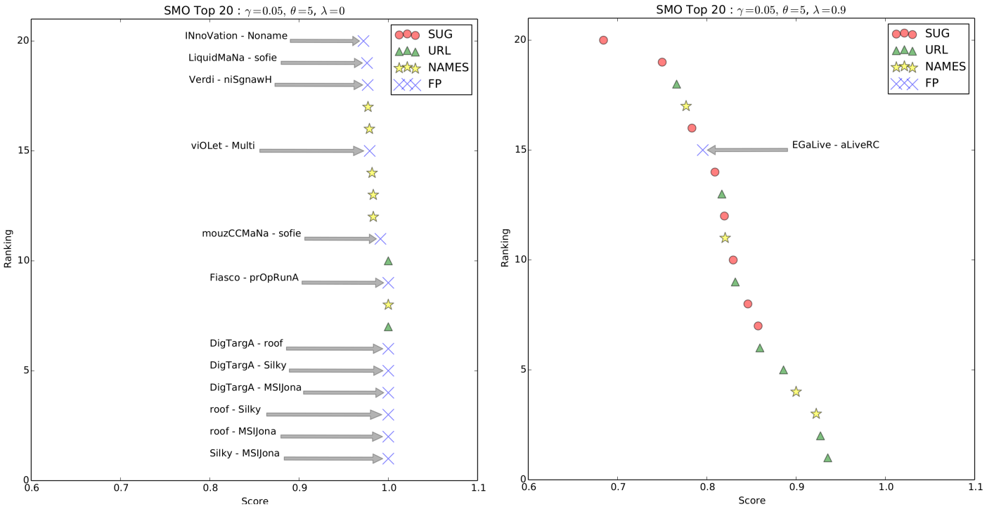
Figure 3: Candidate pairs ranking with \lambda = 0 (left) and with \lambda = 0.9 (right)
