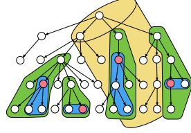
FIG. 1 – Beam search.
