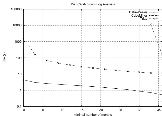
Figure 5: Comparison w.r.t. CUBEMINER and TRIAS (real data)
