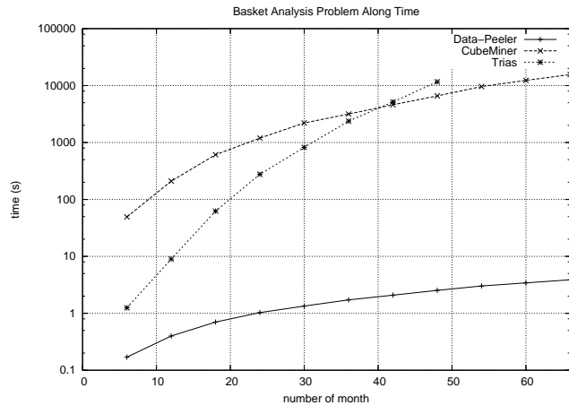
Figure 4: Comparison w.r.t. CUBEMINER and TRIAS
