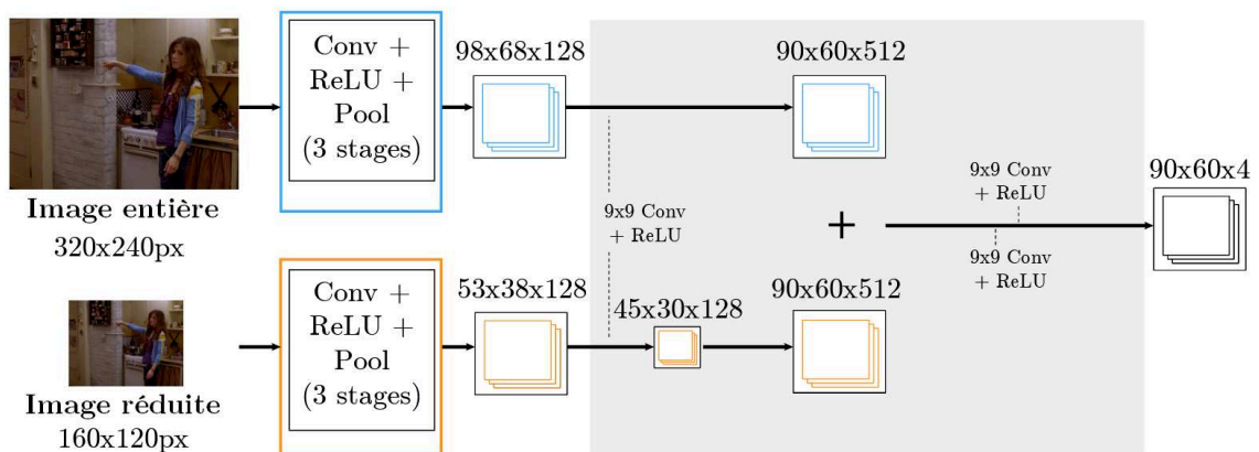
FIGURE 2.19 – Schéma de l’architecture ConvNet Pose (Tompson et al., 2014).
