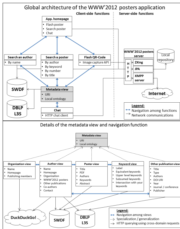
Figure 2. Schemas of the application architecture (cf. http://iris.cnrs.fr/lionel.medini/wiki/doku.php?id=www2012-posters-app-architecture for larger version).
