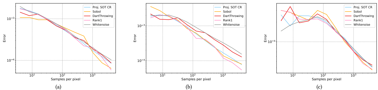
Fig. 15. Convergence plots for 8D. For the three pixel windows depicted in Fig. 11(right), we plot the graphs of absolute errors as a function of sample count.
