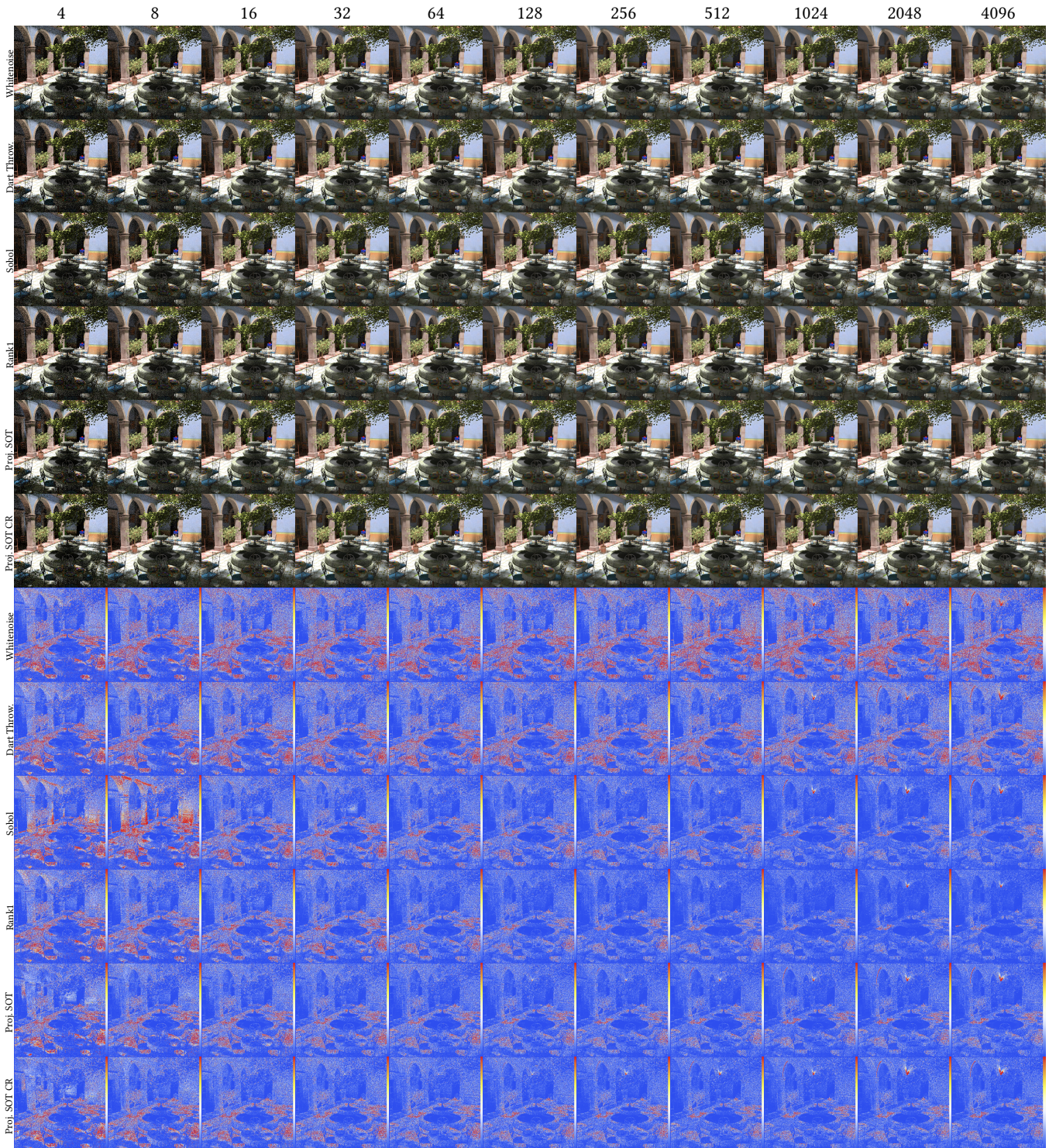
Fig. 10. Rendering with 8D sampling. San Miguel scene with 2 bounces and indirect lighting; absolute error measured with respect to reference image. Colormaps: from blue = 0, to red = 0.0005/spp .
