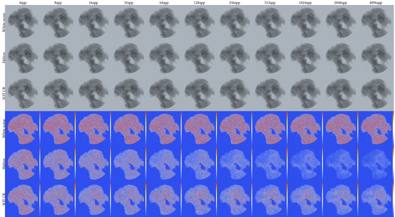
Fig. 11. Extra volumetric rendering results in 8 dimensions (two bounces). Complement of Fig. 17 in the main paper.
