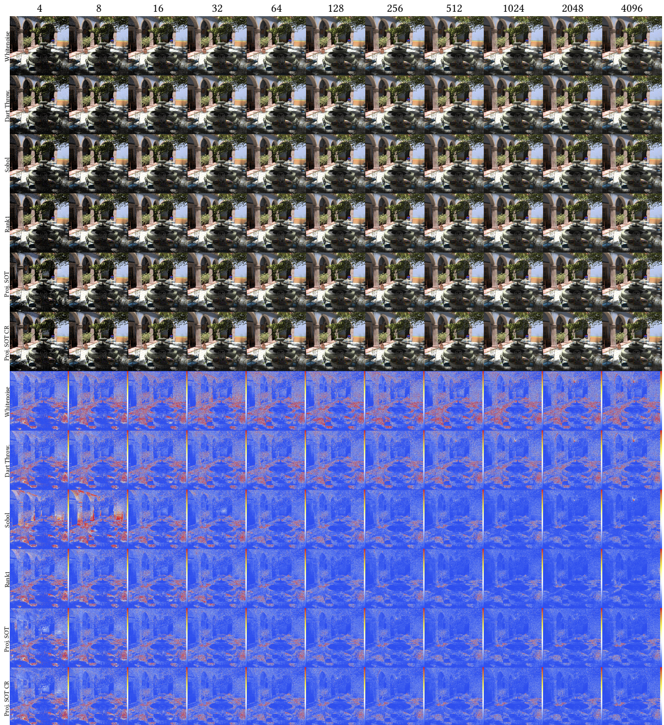
Fig. 8. Rendering with 6D sampling. San Miguel scene with 1 bounce and indirect lighting; absolute error measured with respect to reference image. Colormaps: from blue = 0, to red = 0.0005/spp .
