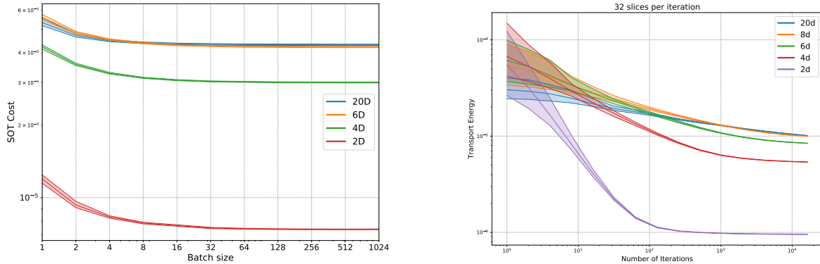
Fig. 3. SOT energy during optimization. Evolution of sliced optimal transport energy of 1024 samples and 64 realisations (mean, min and max plots) as a function of (left) the number of slices per batch for 4096 batches, and (right) the number of batches for 32 slices.
