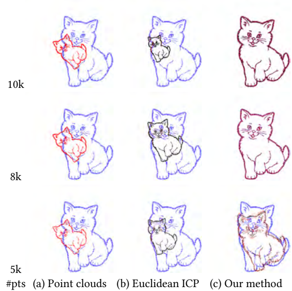
Fig. 8. We compare classical ICP with our method when reducing the number of points being matched. The target distribution always has 10k samples, but we vary the source distribution from 5k to 10k samples. We observe that matching point clouds of similar cardinality behave better: convergence speed increases, and local minimas are less frequently encountered.
