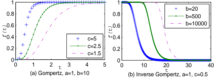
Figure 7: The output of Gompertz and Inv. Gompertz functions
