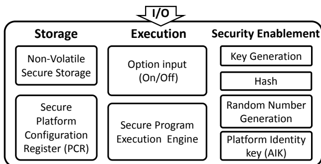
Figure 4: TPM module
