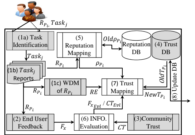
Figure 5: A framework of reputation-based trust system
