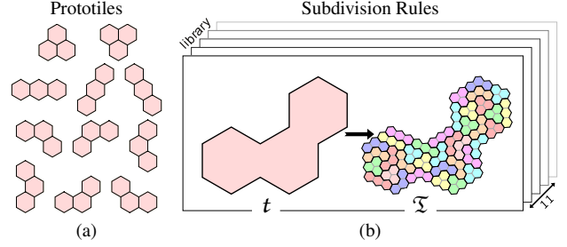
Figure 5: (a) 11 configurations of trihexes on \mathbb{H} . (b) The library of subdivision rules \{t \rightarrow \mathcal{T}\} , where the quasi-trihex tile associated with t after subdivision is partitioned into a set of \lambda = 37 trihexes.
