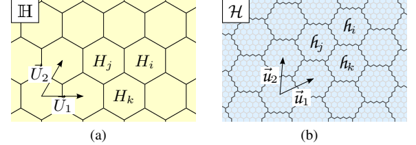
Figure 3: Quasi-hexagonal tiles. (a) The unbounded, regular hexagonal lattice \mathbb{H} generated by (\vec{U}_1, \vec{U}_2) . (b) The unbounded, quasi-hexagonal lattice \mathcal{H} over the finer regular hexagonal lattice \mathbb{h} and generated by (\vec{u}_1, \vec{u}_2) . Each regular hexagon H_i in \mathbb{H} corresponds, through subdivision, to a hextile h_i made up of \lambda small hexagons.
