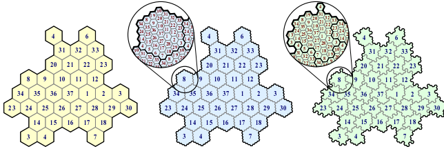
Figure 7: From an irregular hextile \tilde{h}_i with indexed hexagons (left), we apply one regular subdivision step to construct sub-hexagons \tilde{h}_i (center). Replacing each of these \lambda sub-hexagons with a different irregular hextile from \tilde{\mathcal{H}} creates a seamlessly subdivided irregular hextile (right).
