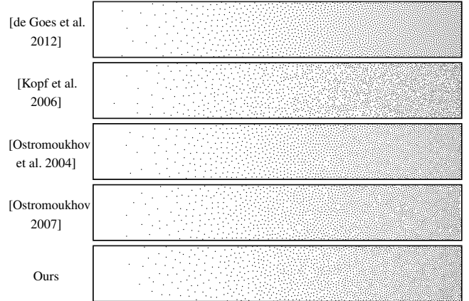
Figure 11: Adaptive sampling of a quadratic density ramp with 2000 points for various sampling algorithms.
