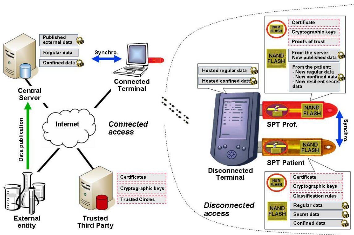
Figure 2: Functional architecture
