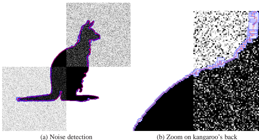
Fig. 10 Noisy contour and noise detection along it by the method of [28]. The input image has been damaged by two different Gaussian noises in different regions. The thresholded shape has a boundary which is damaged in these regions (noisy contour in red). The detector indicates for each contour point what is the local scale at which this part of the contour should be analyzed: the scale or noise level at a point is indicated by the size of the light blue box around it. It is worthy to note that the noise level is almost everywhere proportionnal to the amount of contour degradation.
