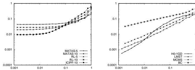
(e) The shape is the accflower (in \mathbb{X}^{\infty-PW-SC} ) digitized for steps h \in [0.001, 1] .
