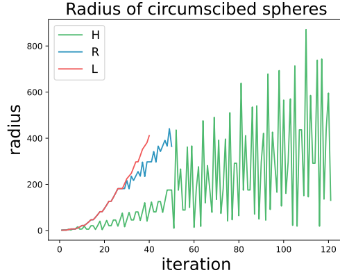
Figure 4: Evolution of the radius of the balls circumscribing two consecutive triangles for a digital plane of normal (2, 5, 156) with H-algorithm (green), R-algorithm (blue) and L-algorithm (red). Only L-algorithm has non-decreasing variation.
