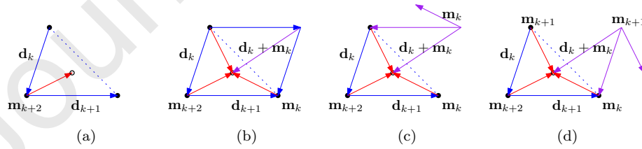
Figure 12: Illustration of Lemma 18 in (a), Lemma 19 in (b) and Lemma 20 in (c) and (d).
