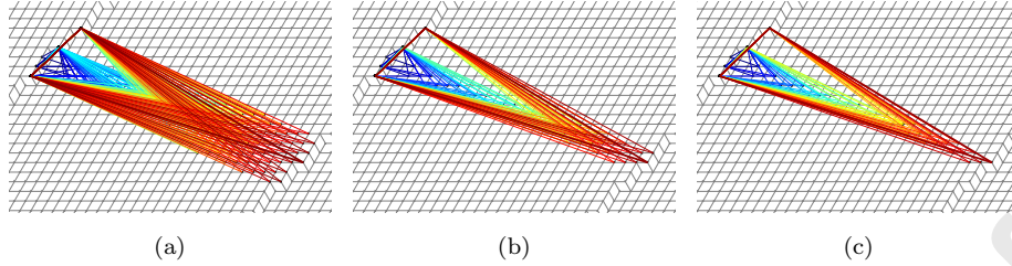
Figure 3: The evolution for normal (2, 5, 156) with H-algorithm (a), R-algorithm (b) and L-algorithm (c). The notations are the same as Fig. 2
