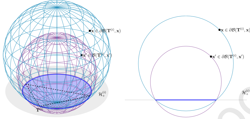
Figure 6: Illustration of the balls \mathcal{B}(\mathbf{T}^{(i)}, \mathbf{x}') (purple) and \mathcal{B}(\mathbf{T}^{(i)}, \mathbf{x}) (blue). Since (\mathcal{B}(\mathbf{T}^{(i)}, \mathbf{x}') \cap \mathcal{H}_+^{(i)}) lies in (\mathcal{B}(\mathbf{T}^{(i)}, \mathbf{x}) \cap \mathcal{H}_+^{(i)}) , we have \mathbf{x}' \leq_{\mathbf{T}} \mathbf{x} .
