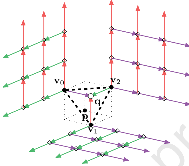
Figure 5: Illustration of the neighborhood \mathcal{N}^{(i)} (marked with hollow diamonds)
