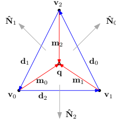
Figure 9: Notations for \mathbf{v}_k (black), \mathbf{m}_k (red) and \mathbf{d}_k (blue). Note that \hat{\mathbf{N}}_k (grey) is used only in sec. 5.1.
