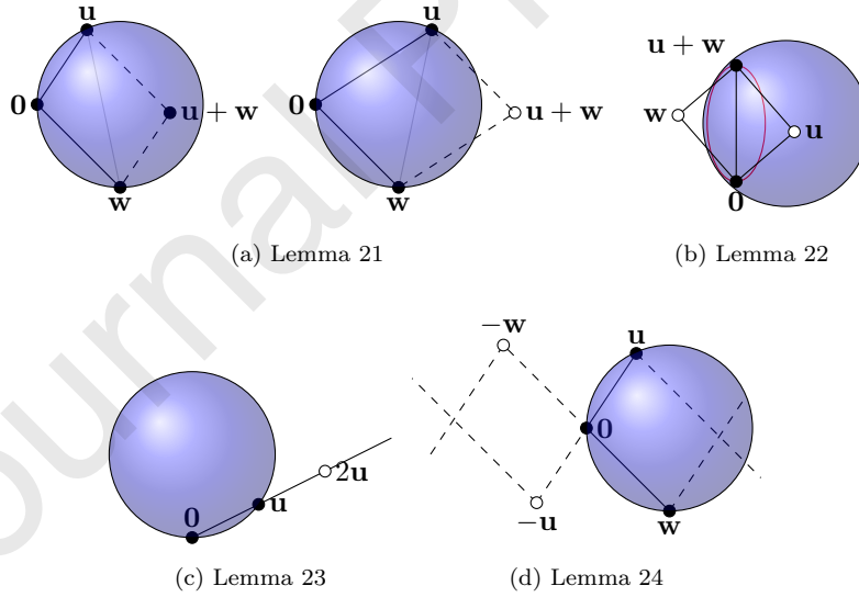
Figure 13: Illustrations for circumsphere-based lemma of sec. 5.2. A point is depicted as a black disk if it is inside the ball of interest, and as a hollow disk if it is not in the closed ball.
