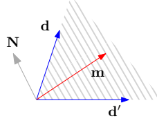
Figure 11: Illustration of Lemma 17. Note that \mathbf{m} does not belong to the span of \mathbf{d} and \mathbf{d}' . However, it projects along \mathbf{N} into the interior of the convex combination of \mathbf{d} and \mathbf{d}' (hatched area).
