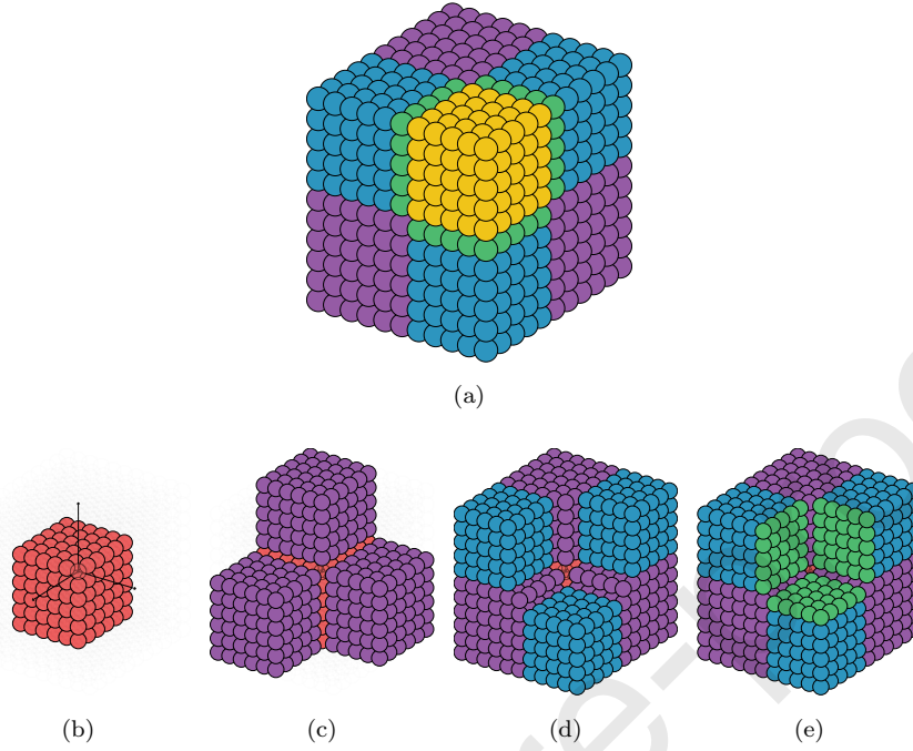
Figure 8: The discrete space \mathbb{Z}^3 (intersected with the box [-5, 5]^3 for the illustration) is partitioned into five regions: the yellow, green, blue and purple regions respectively correspond to (Case 1), (Case 2), (Case 3) and (Case 4), the red one is discarded because none of its points lie in \mathcal{H}_+ (the three black arrows indicate the direction of the grid axes).
