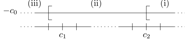
Figure 10: Relative position of -c_0 with respect to c_1 and c_2 . Three separate cases, (i), (ii), and (iii), are considered in the proof.
